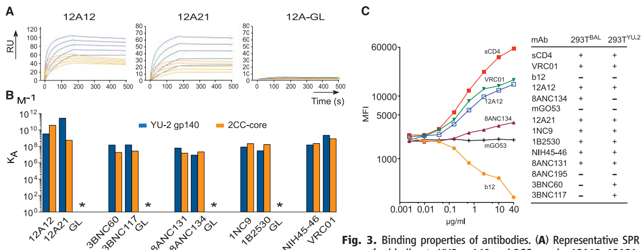
Fig. 3. Binding properties of antibodies. (A) Representative SPR sensorgrams for binding to YU2-gp140 and 2CC core by 12A12, 12A21 (Fig. 2B and table S5), and 12A germ line (GL)-reverted antibodies. (B) Graph shows K_A for representative antibodies (tables S5 and S9). (C) Graph shows mean fluorescence intensity of CD4i antibody 3-67 (7) binding to Bal-expressing 293T cells after incubation with the indicated antibodies. Table indicates whether or not an antibody induces CD4i site accessibility (fig. S11).
